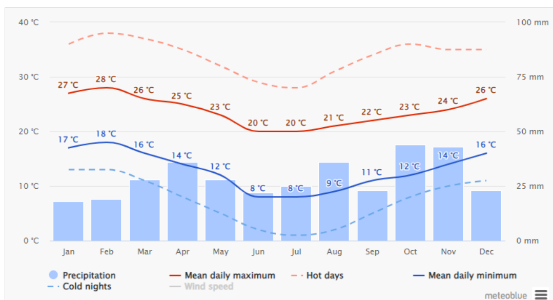
Figure 6. Summary of historical climate (modelled) for Brenton on Sea ( www.meteoblue.com ).
