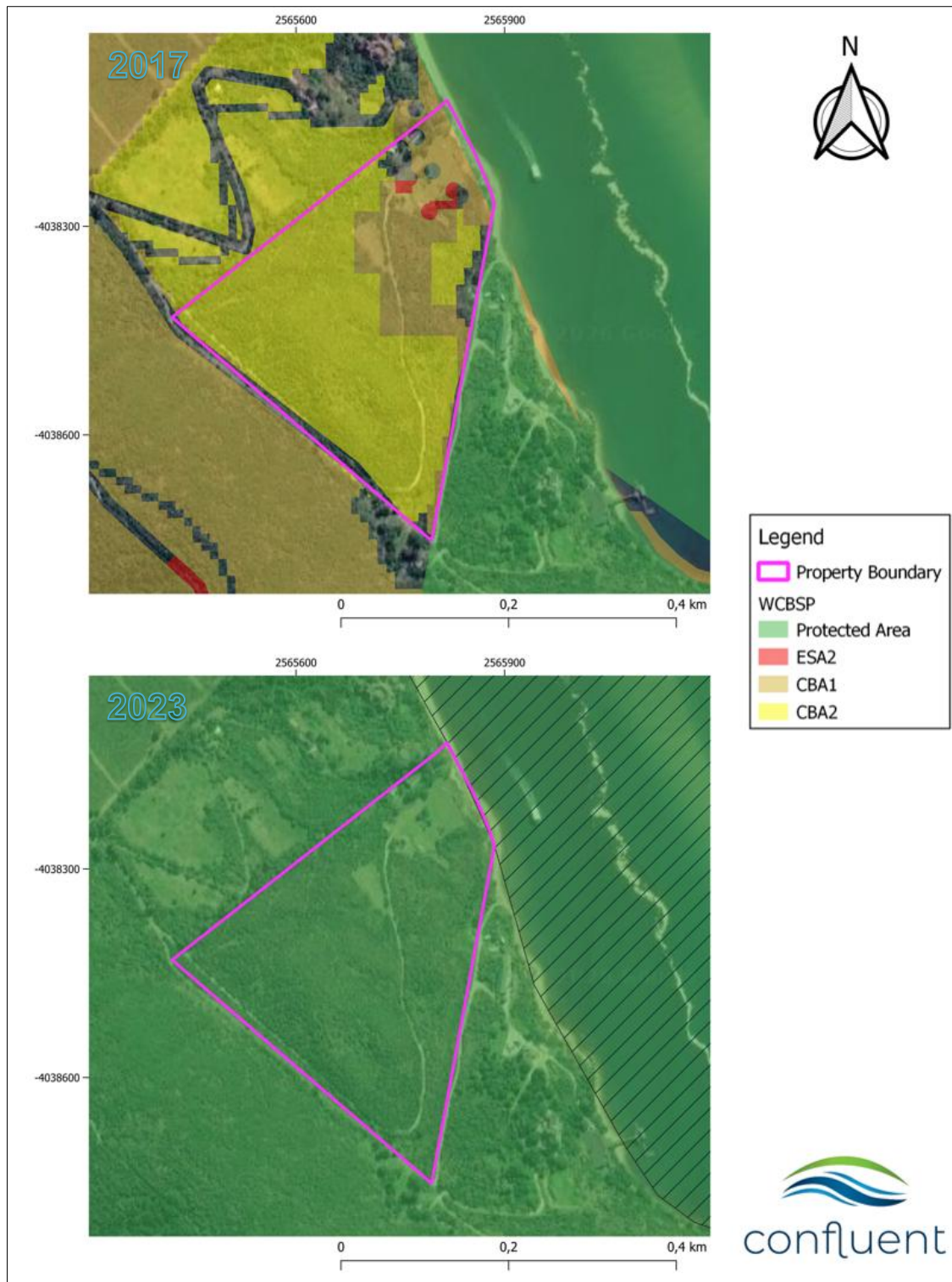
Figure 8. Site map of Portion 104 of Uitzigt Farm 216 with layers for the Western Cape Biodiversity Spatial Plan layers for 2017 (above) and 2023 (below). Knysna Protected Environment as mapped by SANParks is shown using black stripes.
