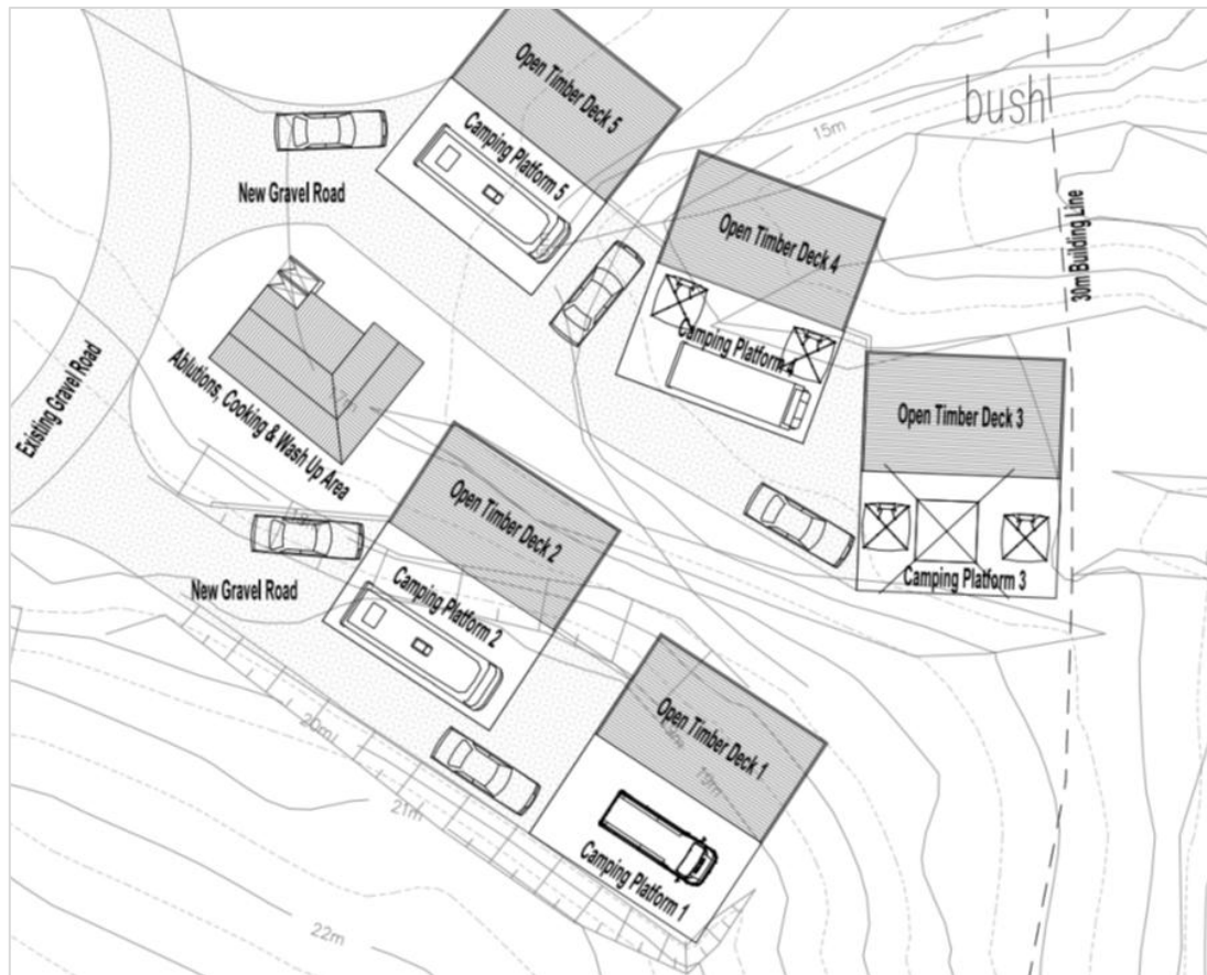
Figure 3. Proposed development layout of one camp area (labelled EUA1 in Figure. 2).
