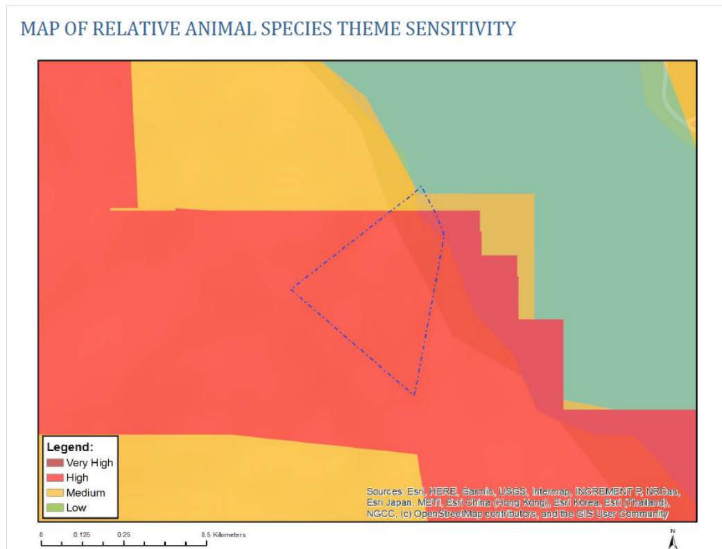
Figure 5. DFFE Online Screening Tool outcome for the terrestrial animal species theme Portion 104 of Uitzigt Farm 216. The property boundary is indicated by the blue dashed line.
