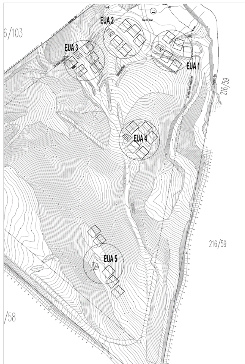
Figure 2. The Site Development Plans (SDP) for Portion 104 of Uitzigt Farm 216 showing 1m contour lines, 25 concrete platforms, their associated timber decks, and 5 ablution blocks proposed for the north of the property.
