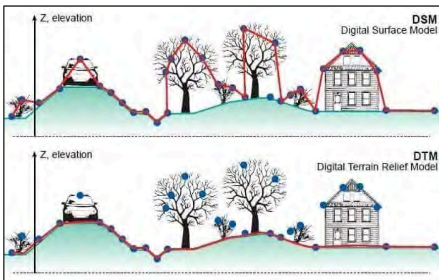
Figure 6: Terrain models
