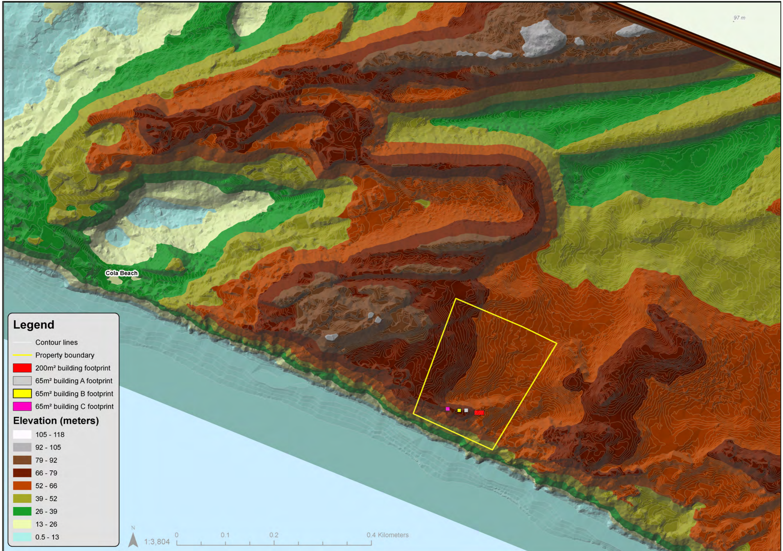
Figure 3: Topography
