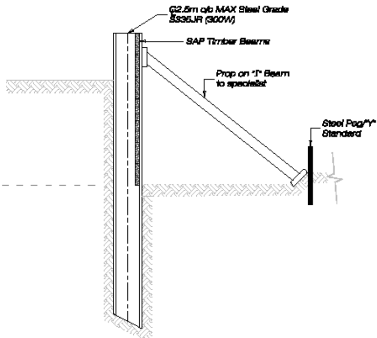
Typical Shoring Detail to minimize environmental damage
