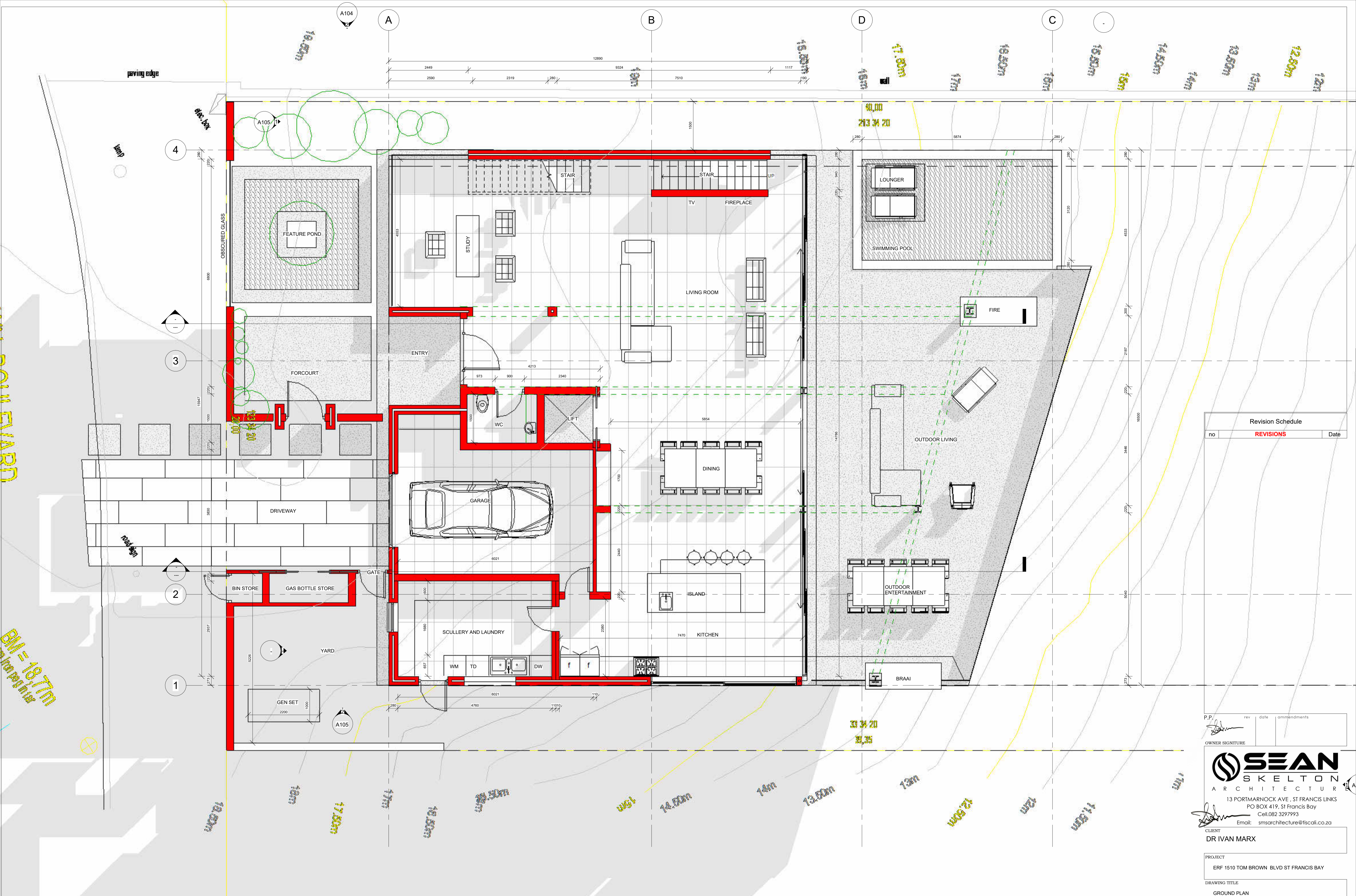
1 GROUND FLOOR LEVEL 1 : 50
